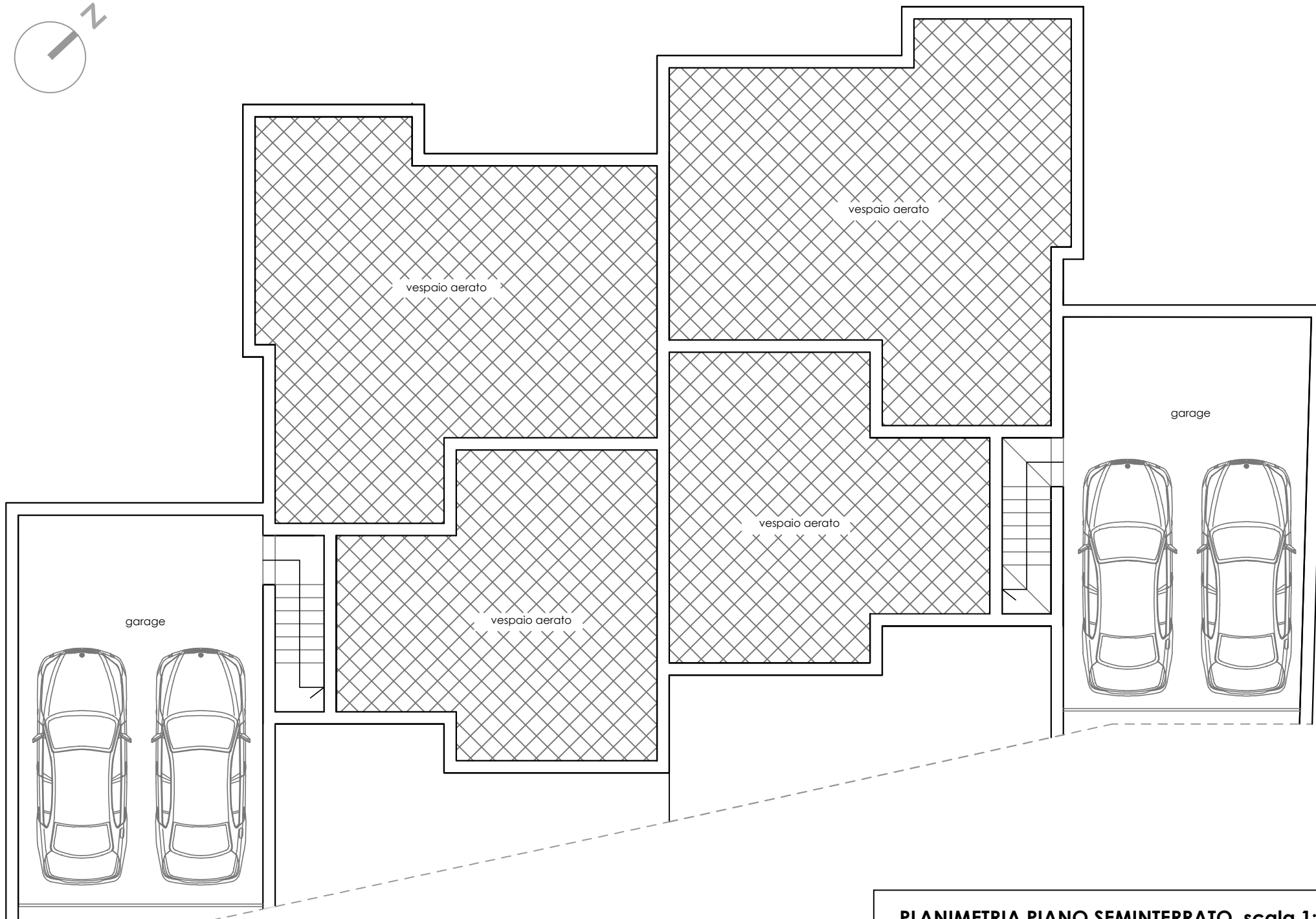
PLANIMETRIA PIANO SEMINTERRATO, scala 1:100
